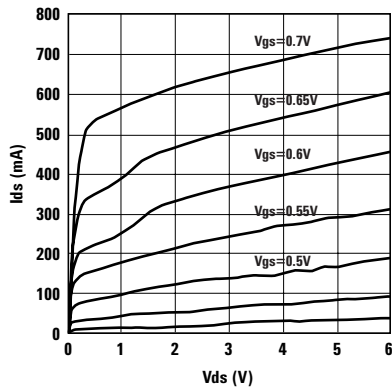
Figure 1. Typical IV curve (V gs = 0.01V) per step.
